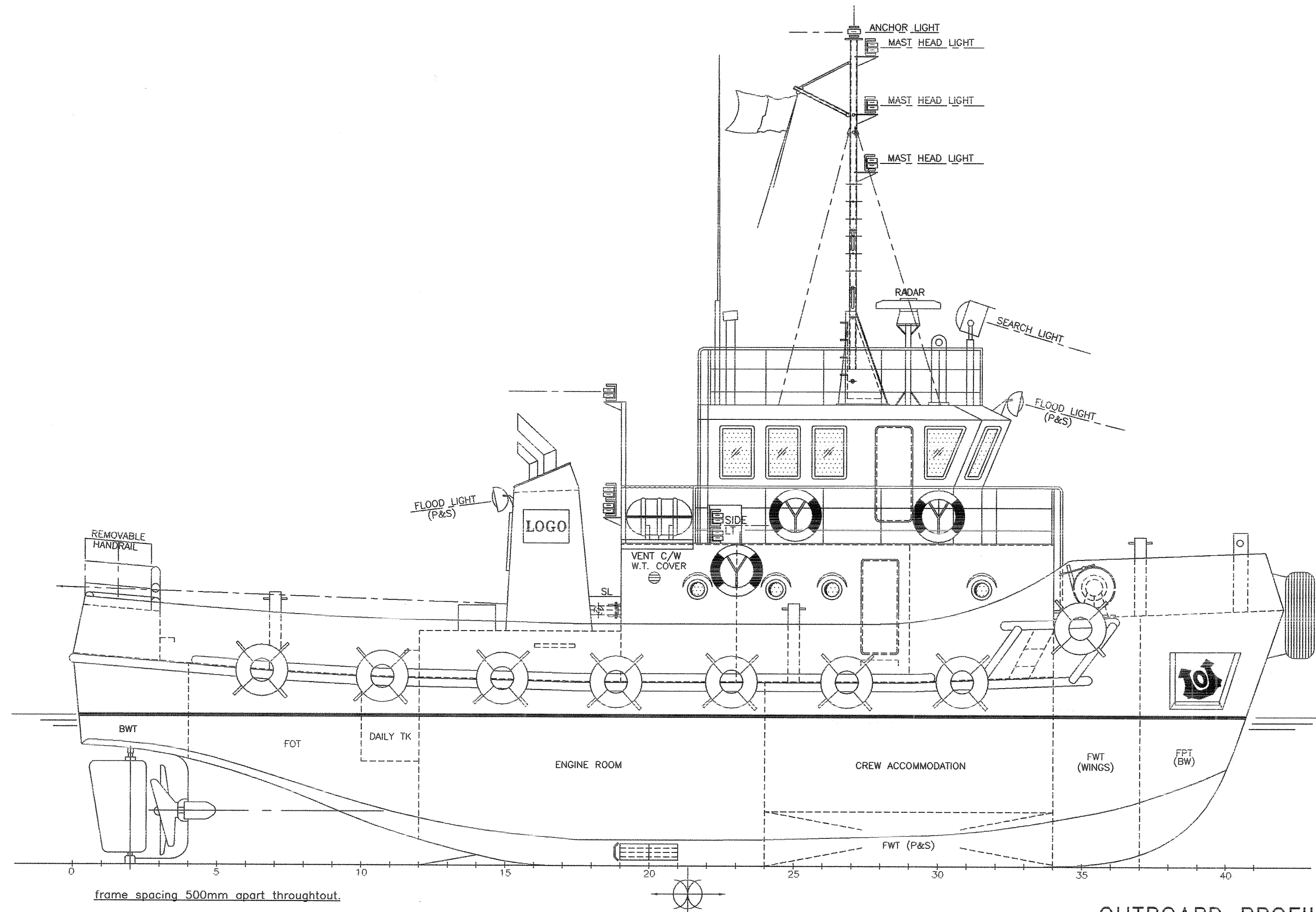
OUTBOARD PROFILE
