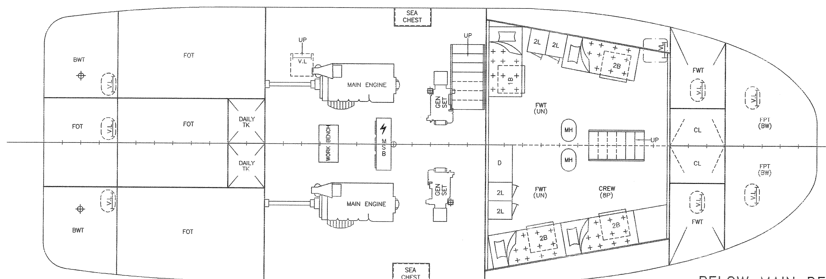
BELOW MAIN DECK
