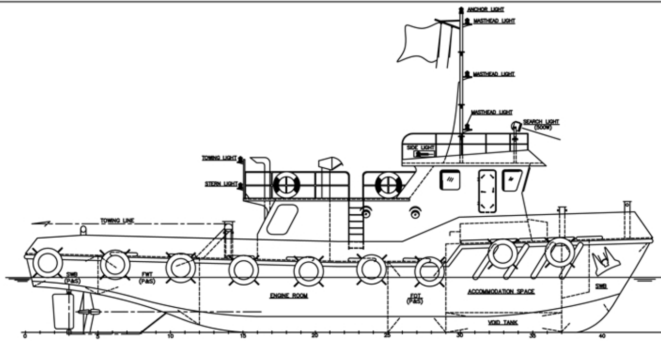
SIDE ELEVATION
