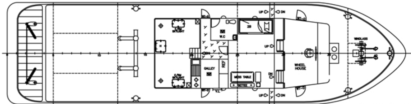
MAIN DECK PLAN
